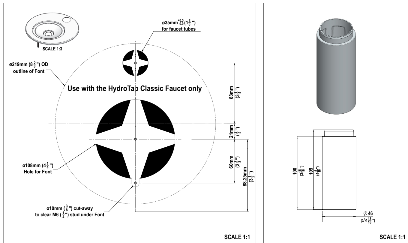
Benchtop Cutting Template for Fonts mounted with HydroTap Classic Faucet
